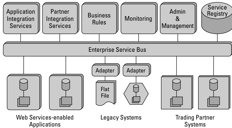
Figure 5-2: The Enterprise Service Bus architecture
