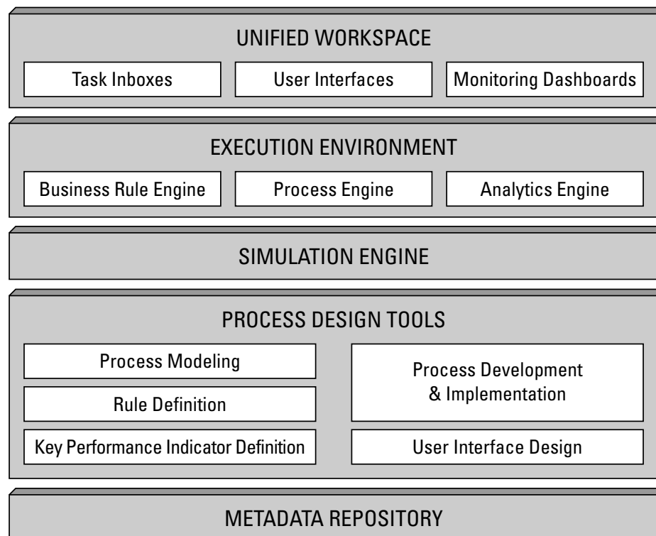
Figure 5-1: The BPM technology architecture.
